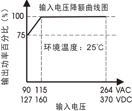
LOF550-20Bxx 输入电压降额
