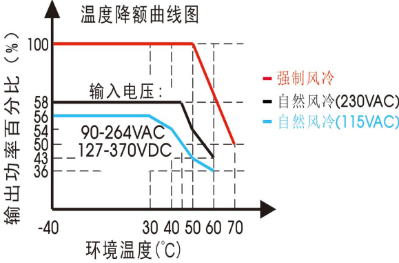
LOF550-20B24/27/36V/48/54 (满载 550W 带 25CFM 风扇)
